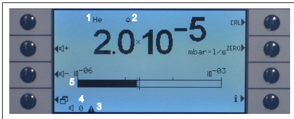
Fig. 3-3 Measurement screen with leak
