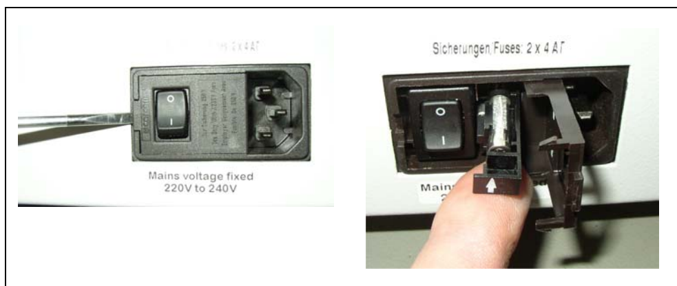
Fig. 7-4 Replacing the mains fuse
