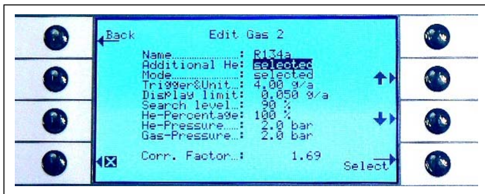
Fig. 4-3 Selecting additional Helium
