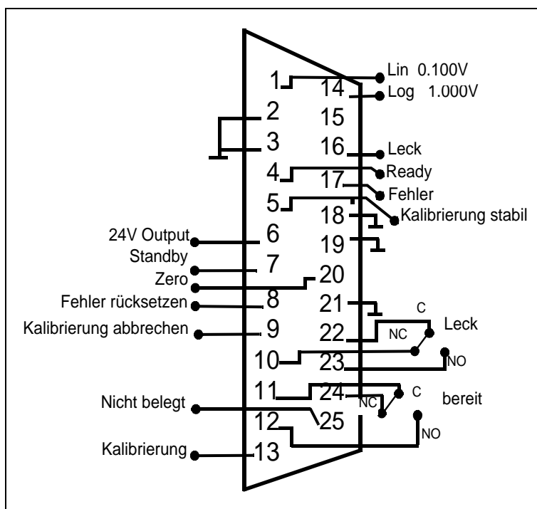
Fig. 6-1 Default Pin Assignment
