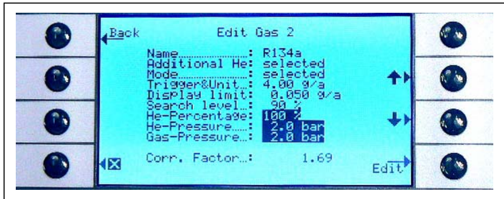
Fig. 4-5 Setting a refrigerant equivalent correction factor
