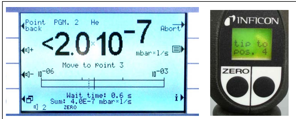
Fig. 3-11 •Guide screens requesting the next location
