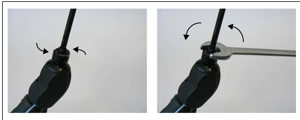
Abb. 7-10 Switching of the handle and sniffer tip - without or with wrench
