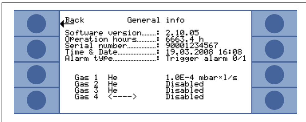
Fig. 3-14 Info page without errors or warnings
