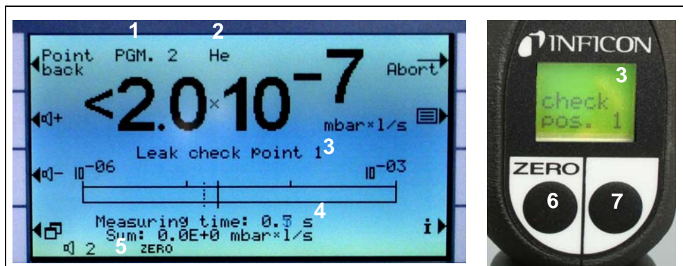
Fig. 3-10 I•Guide screens during measurement
