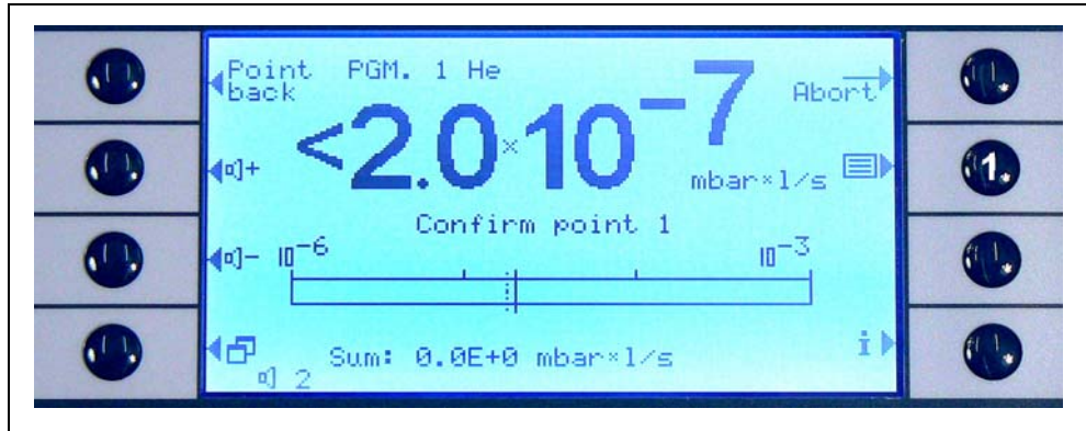
Fig. 3-8 Measuring Screen in I•Guide Mode
