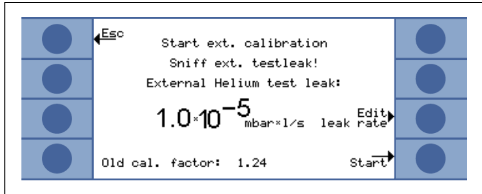
Fig. 3-19 Setting-up the leak rate of the external leak
