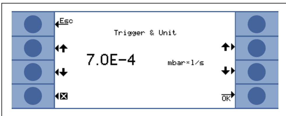
Fig. 4-7 Setting-up trigger level and unit of measurement
