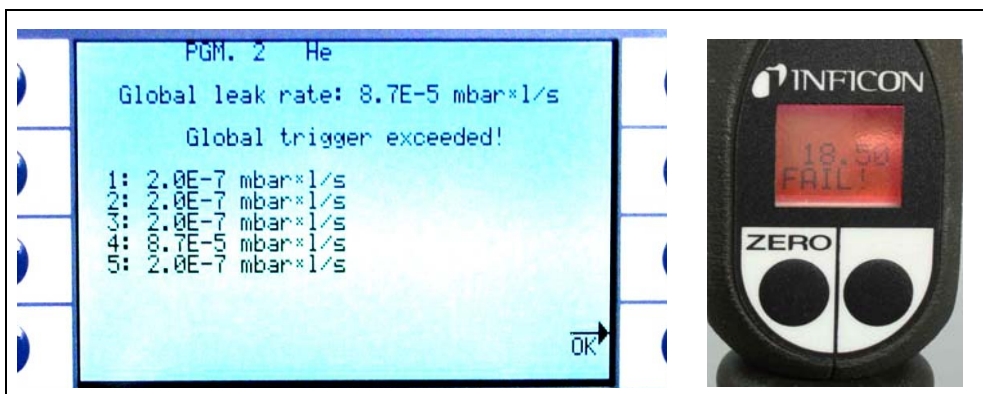
Fig. 3-13 Result of I•Guide program: unit under test failed
