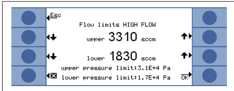
Fig. 4-12 Variation of flow limits
