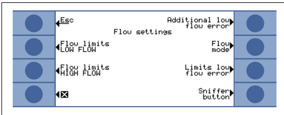
Fig. 4-11 Setting up flow settings
