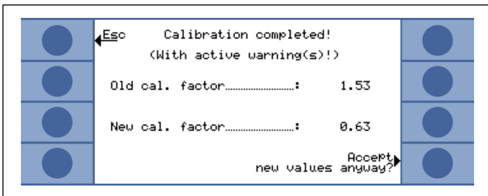
Fig. 3-22 Results of external calibration
