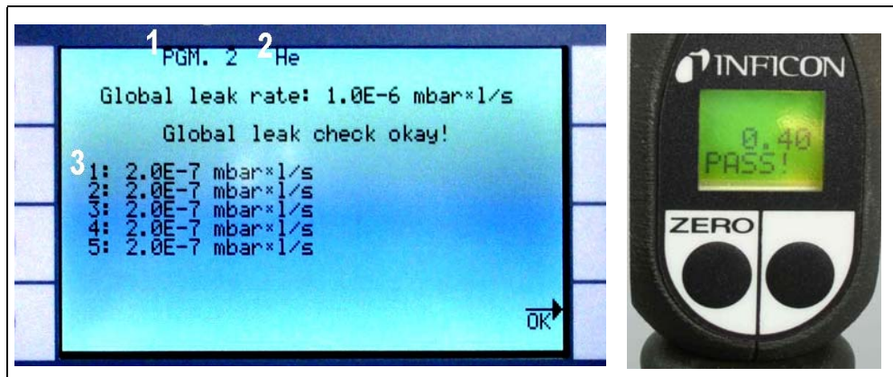
Fig. 3-12 Result of •Guide program: unit under test passed
