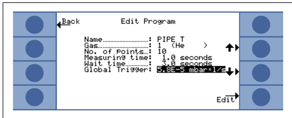
Fig. 4-18 Editing an I•Guide program
