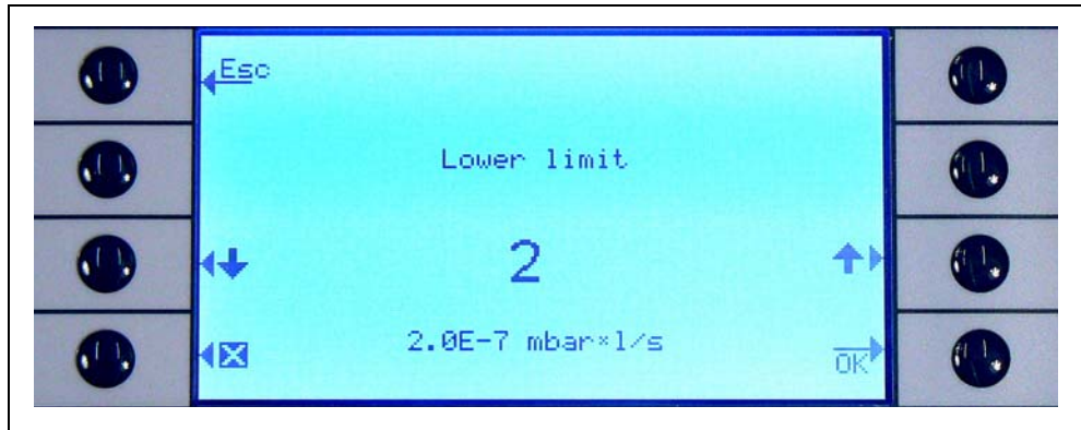
Fig. 4-8 Editing the lower display limit
