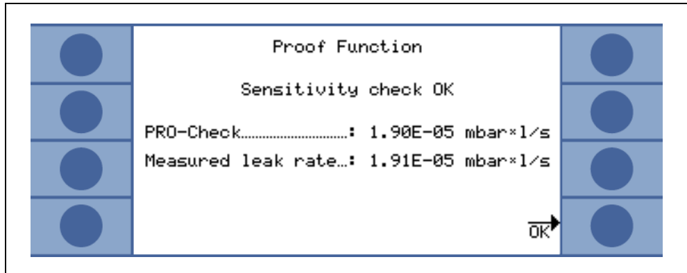
Fig. 3-16 Results of proof function for Protec P3000
