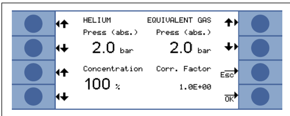
Fig. 4-6 Editing parameters for refrigerant equivalent leak rates
