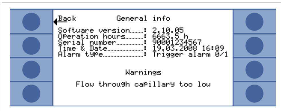
Fig. 3-15 Info page with active warning
