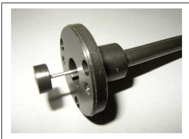
Fig. 7-16 Steel capillary sticking out of sniffer tip flange
