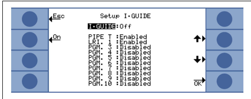
Fig. 4-17 Setting-up the I•Guide Mode
