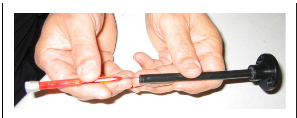
Fig. 7-15 Pushing out the steel capillary
