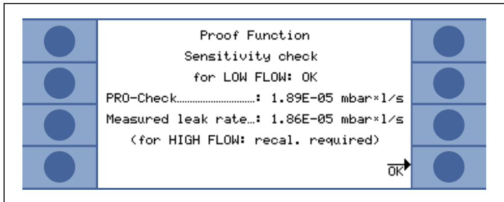
Fig. 3-17 Results of proof function for Protec P3000XL
