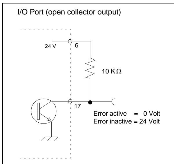
Fig. 6-2 Circuit for open collector output "Error"
