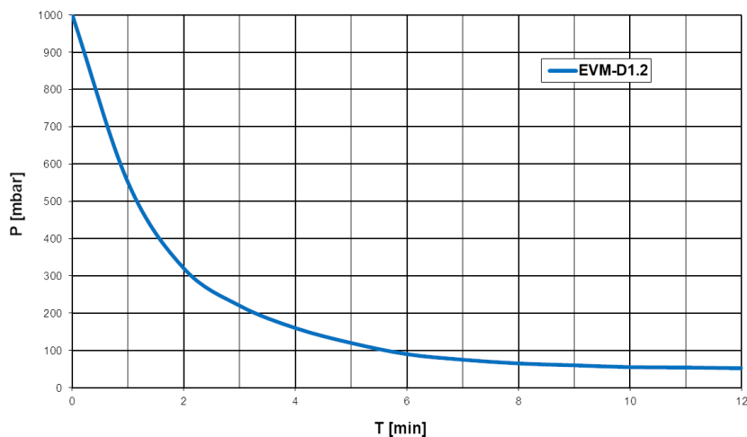
Pumpdown time for 20 ltr vessel
