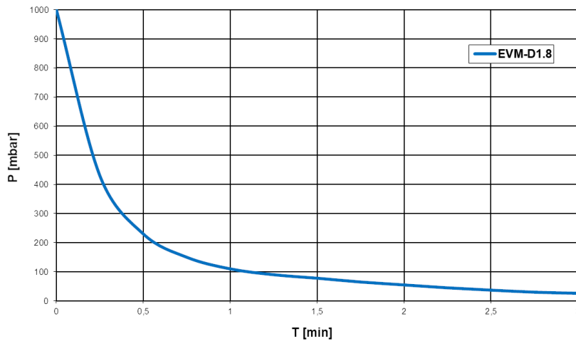
Pumpdown time for 10 ltr vessel
