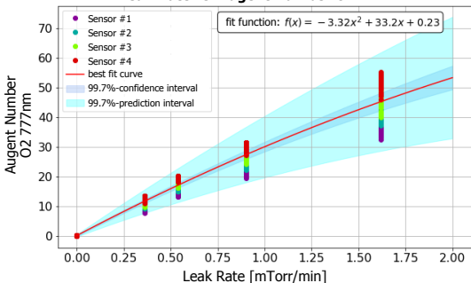
Leak Detection RoR in Helium - pressure 90 mTorr Leak Rate vs. Augent Number O2 777nm
